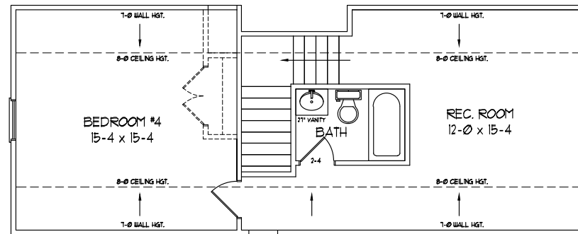
SECOND FLOOR
