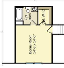
Second Floor Plan 1/4" = 1'-0" (OPTIONAL BONUS W BATH)
