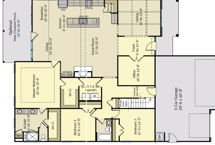
Gourmet Kitchen 1/4" = 1'-0" (OPTIONAL)
