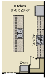
Gourmet Kitchen 1/4" = 1'-0" (OPTIONAL)
