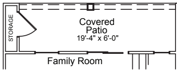
Covered Patio Option
