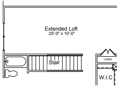
Extended Loft Option I.L.O. UNFINISHED STORAGE
