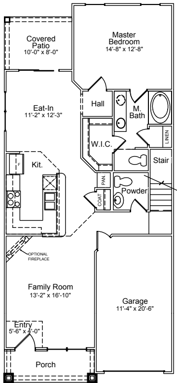
"A" 1st Floor Plan
