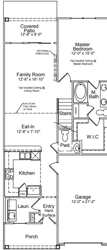
"A" & "B" 1st Floor Plan
