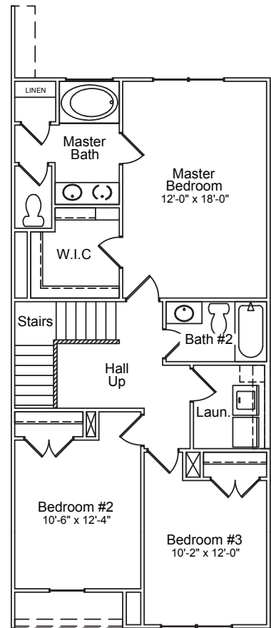
"A" & "B" 2nd Floor Plan
