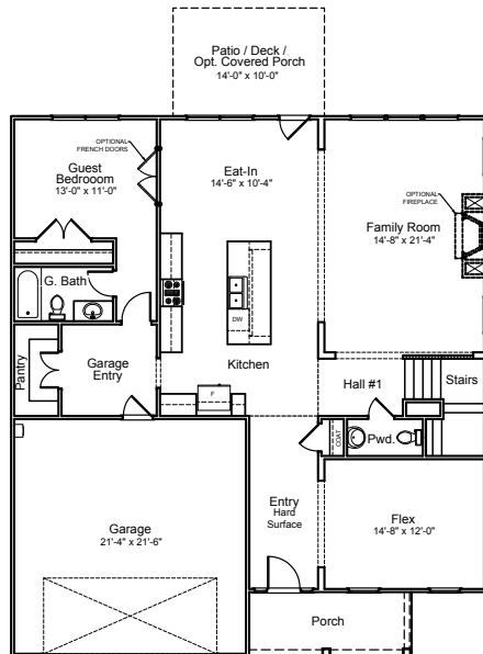
"A" 1st Floor Plan
