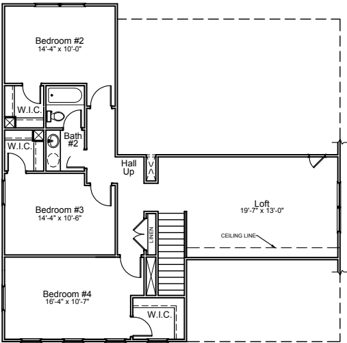
"A" 2nd Floor Plan
