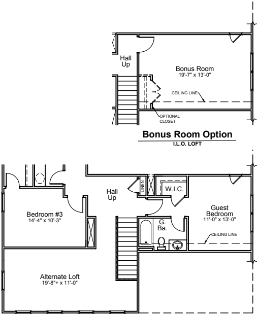
Guest Suite Option
