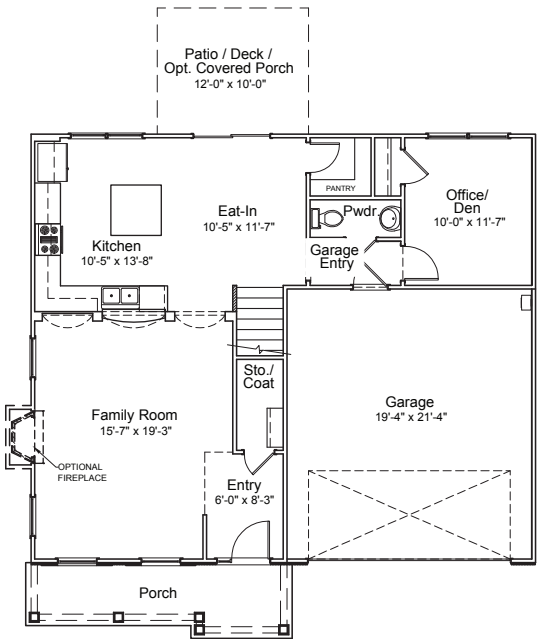
"A" 1st Floor Plan
