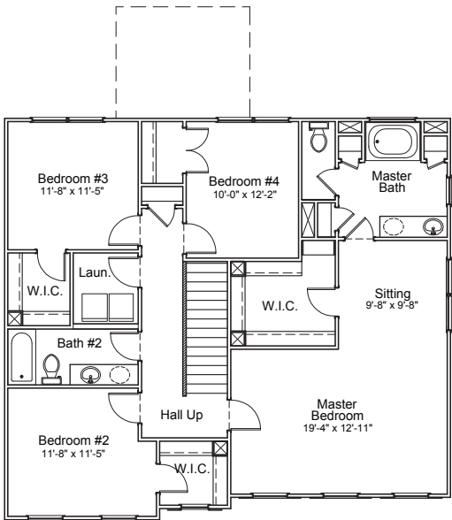
"A" 2nd Floor Plan
