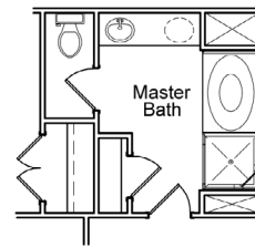
Tub/Shwr Opt. @ Mstr w/ Bonus
