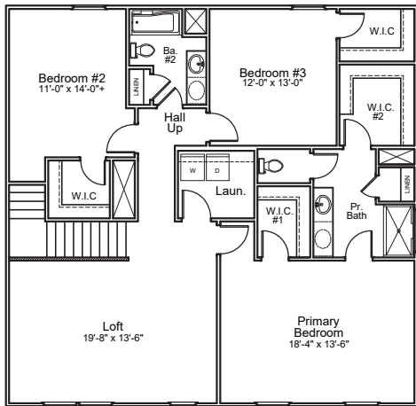
"A" 2nd Floor Plan
