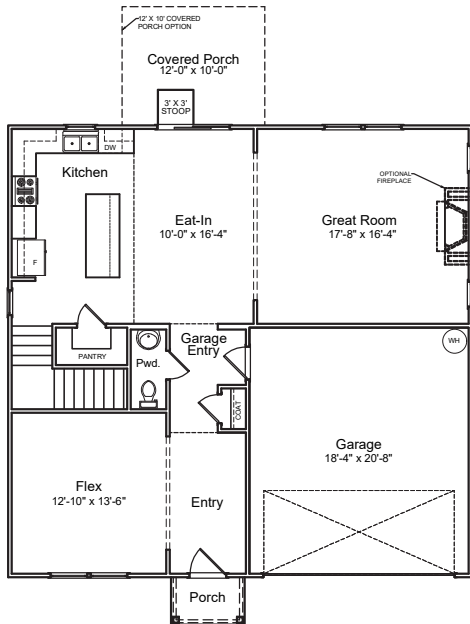
"A" 1st Floor Plan
