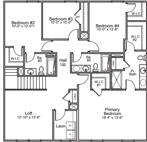
Alternate 2nd Floor w/ 3rd Bath Option
