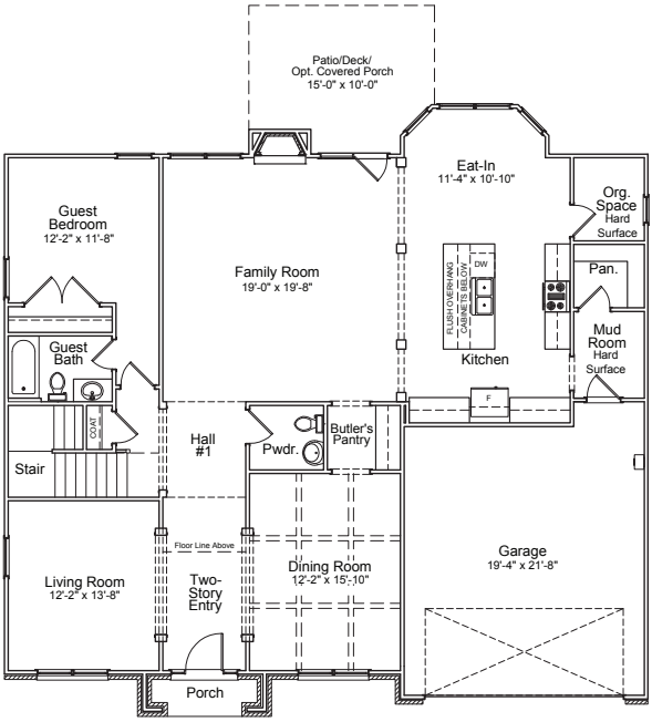
"A" 1st Floor Plan
