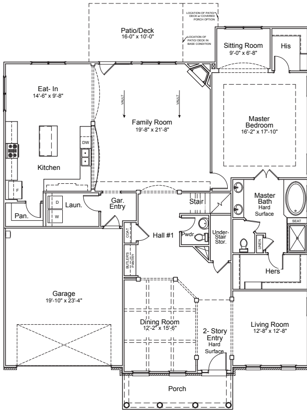
"A" 1st Floor Plan
