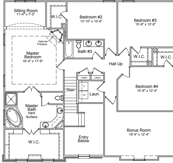
"A" 2nd Floor Plan
