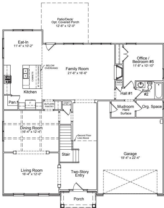
"A" 1st Floor Plan
