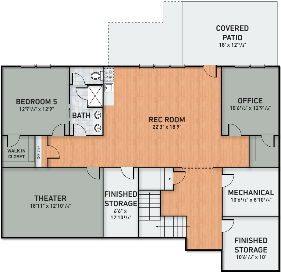
BASEMENT PLAN
