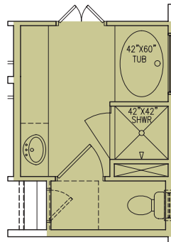
GARDEN TUB 60X42 AND SEPARATE SHOWER – WALL TILE & 42X42 PAN
