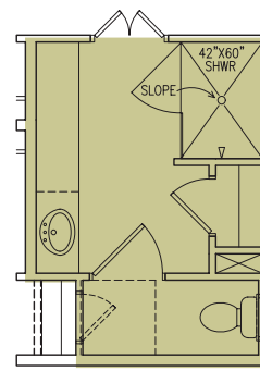
60X42 SHOWER ONLY WALL TILE W/ZERO ENTRY ON SLAB
