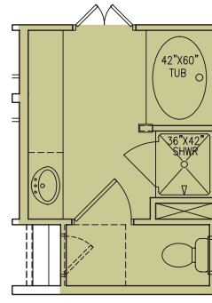
GARDEN TUB 60X42 AND SEPARATE PREFAB SHOWER 42X36
