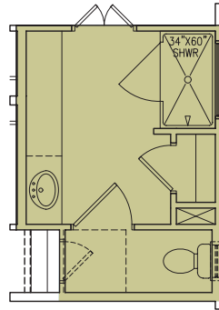
PREFAB SHOWER ONLY 60X34
